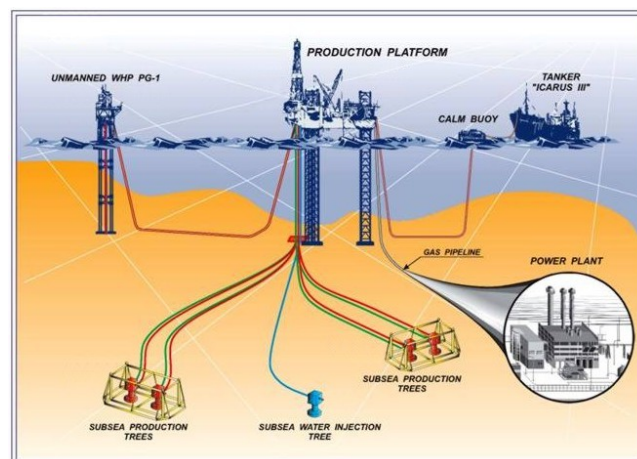
Figure 6. Layout of B3 oilfield infrastructure. http://www.lotos.pl/ Retrieved 05-06-2015.
